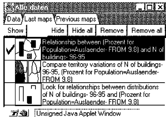
Fig.9. Several different presentations of the same data are differentiated by map names and icons.
